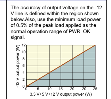
<Fig.4> Min. load condition
