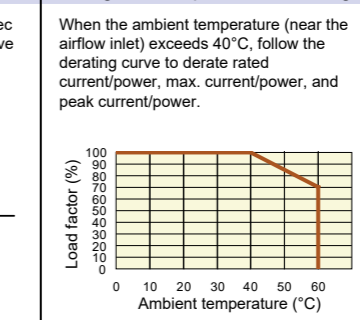
<Fig.3> Temperature Derating
