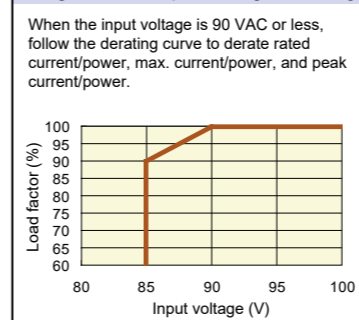
<Fig.1> Low input voltage derating
