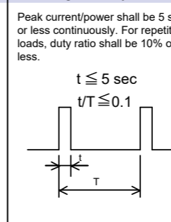
<Fig.2> Duty Ratio
