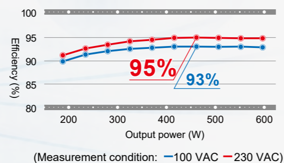
Efficiency graph (UZP-600-A24, an example measurement)
